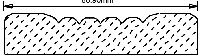
FB35043 3.5" 88.90mm
