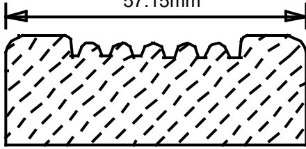
FB22551 2.25" 57.15mm
