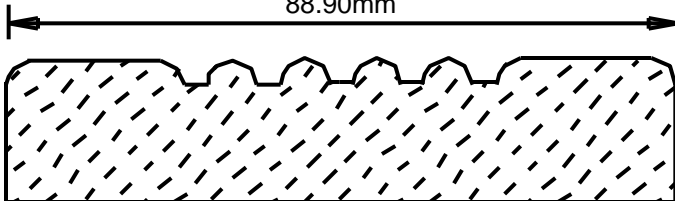
FB35042 3.5" 88.90mm
