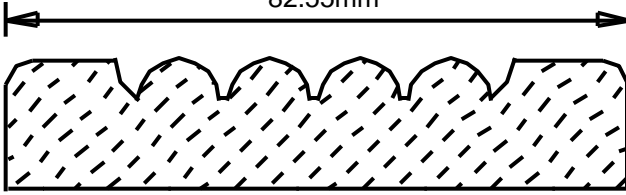
FB32541 3.25" 82.55mm
