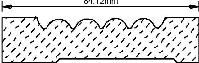
FB33141 3.312" 84.12mm
