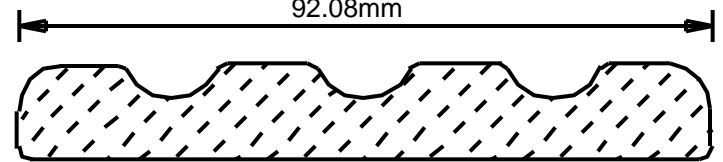
FC36231 3.625" 92.08mm
