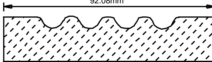
FC42541 4.25" 107.95mm
