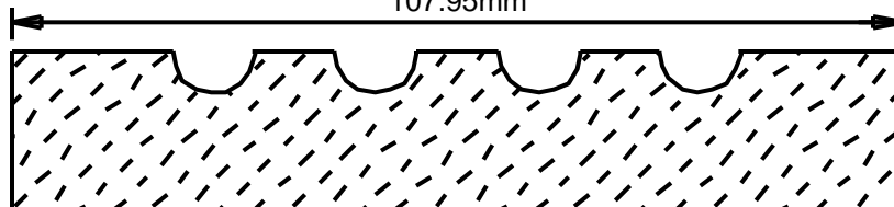
FC42551 4.25" 107.95mm
