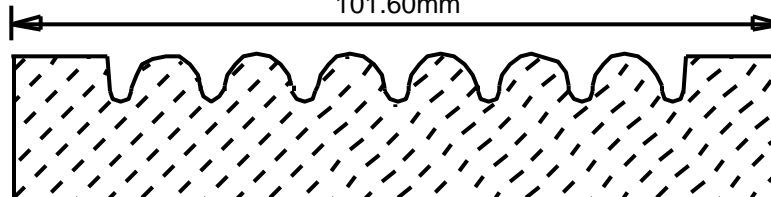
FB40061 4" 101.60mm
