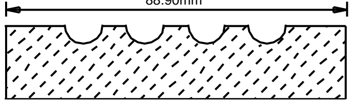
FC35051 3.5" 88.90mm
